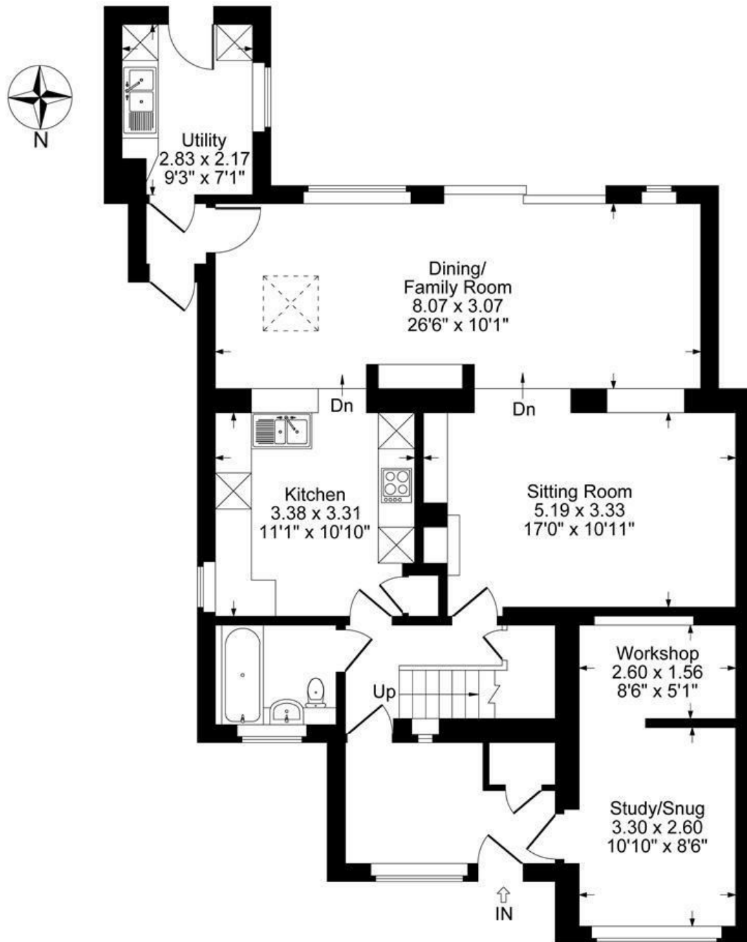
Ground Floor
